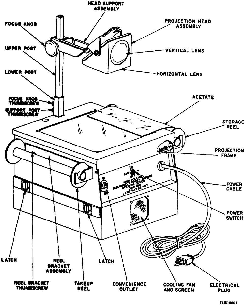
Figure 1-1. Projector, Still Picture PH-637E//PFP. 1-1
