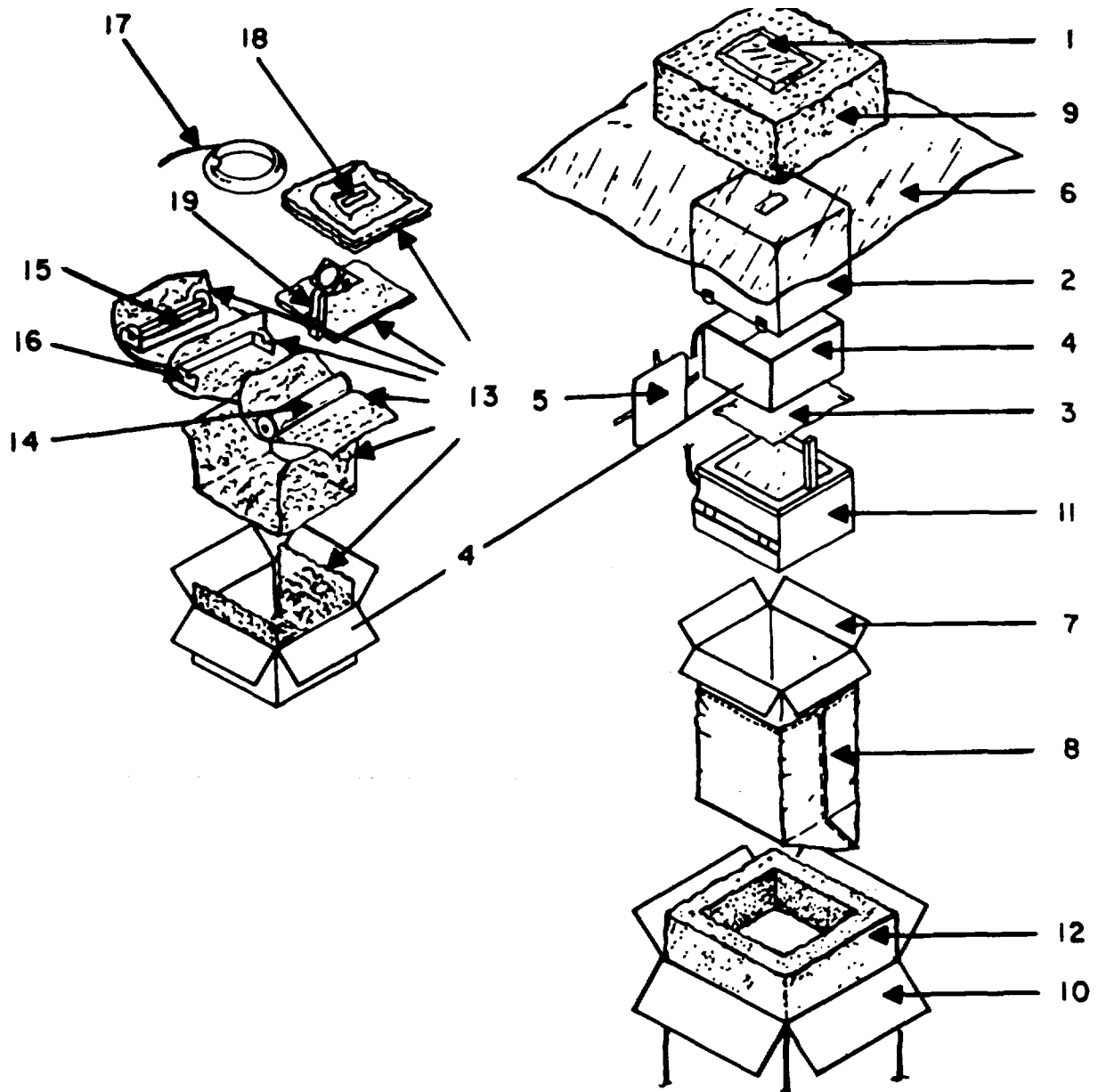
Figure 2-1. Projector, packing diagram. Change 4 2-1
